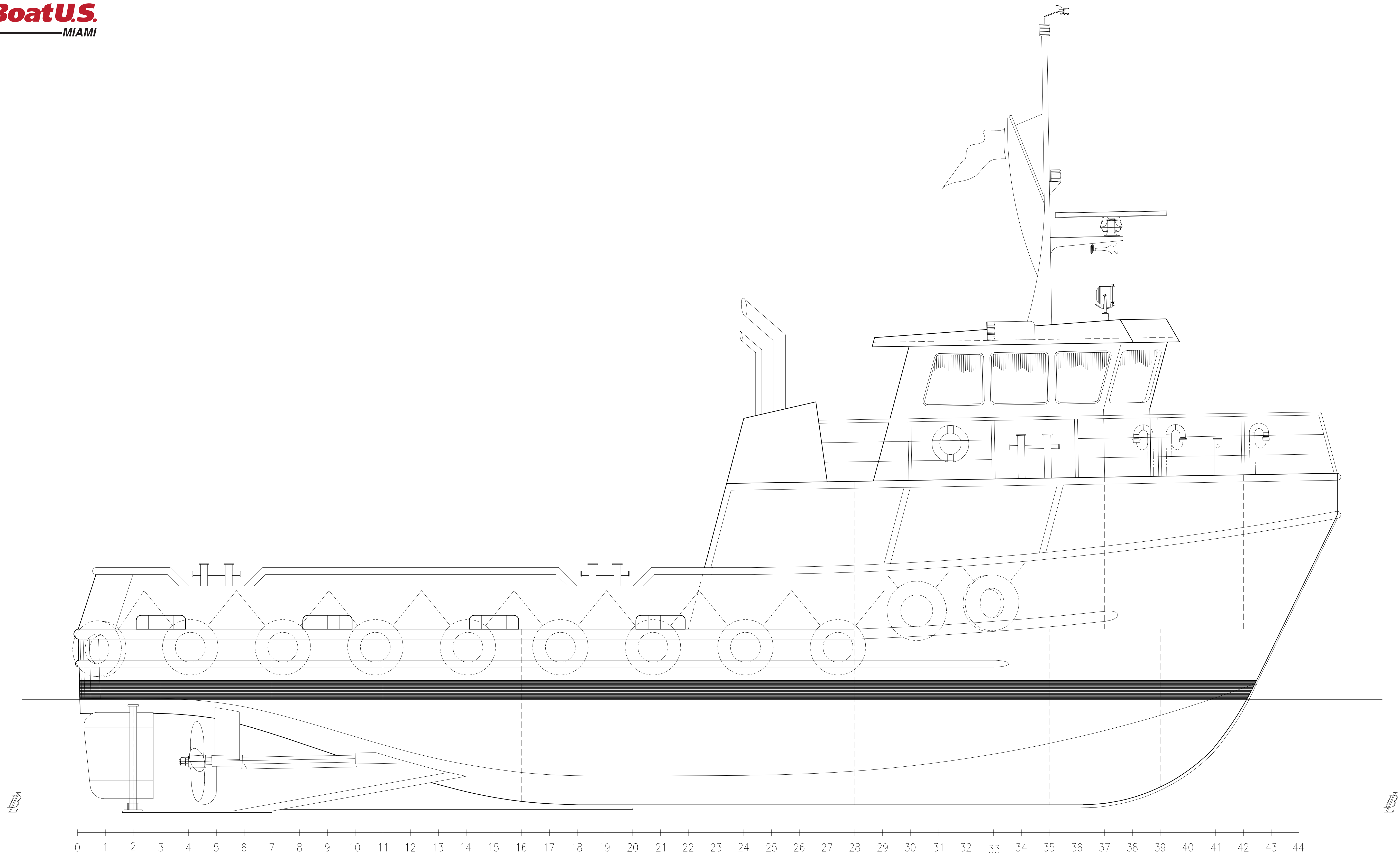
OUTBOARD PROFILE
